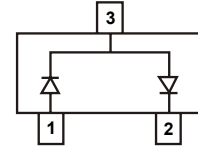
BAT54S Marking : LD3, KL4
